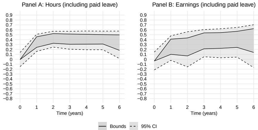
Figure 8: Bounds Measuring Male Income at Same Age as Female
