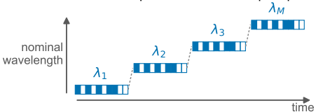
a One code period at each sweep step
