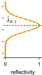
f FBG 2 spectrum
