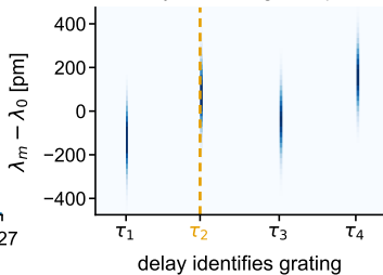
e Delay--wavelength map
