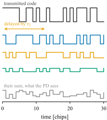
(a) one code period, one wavelength step
