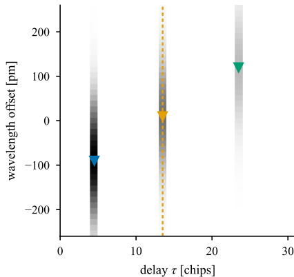
(b) after correlating every row
