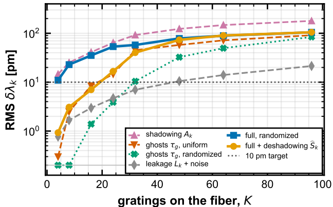
(a) Error mechanisms vs array size, R = 10\%
