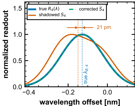
(a) 4th grating behind three, R = 20\%
