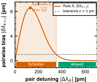
(b) Rule A as a placement criterion
