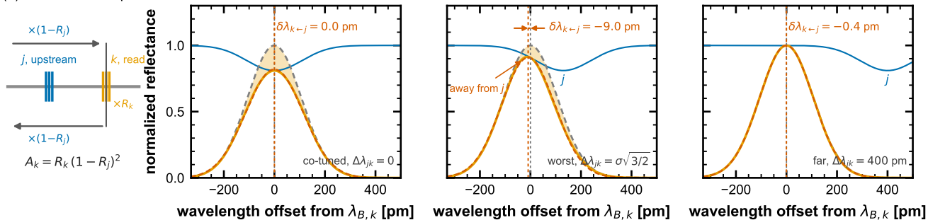
(a) Rule A on the spectrum
