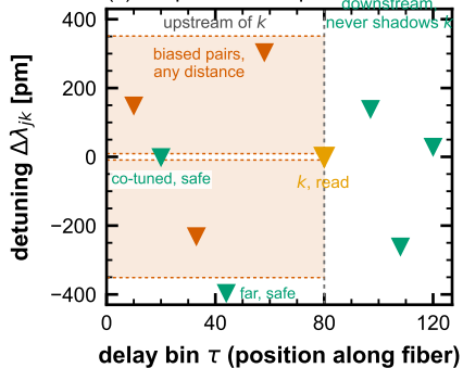
(c) the pairs Rule A prices
