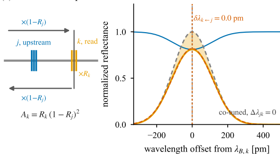
(a) Law A on the spectrum
