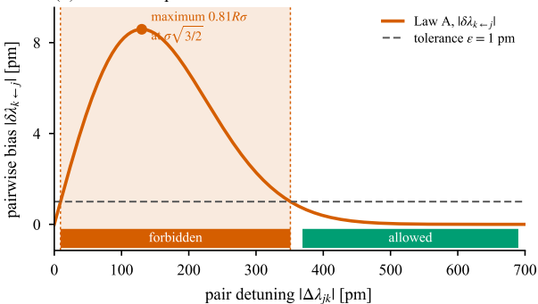
(b) Law A as a placement rule
