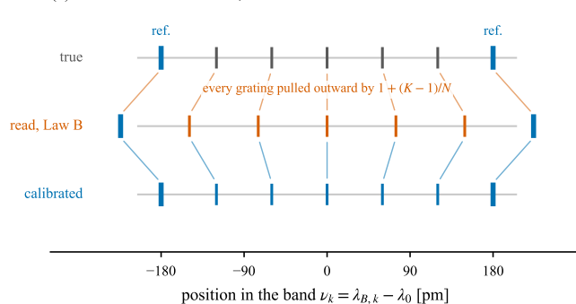
(c) Law B: an axis stretch, two references remove it
