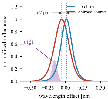
(b) FM-to-AM on the flank
