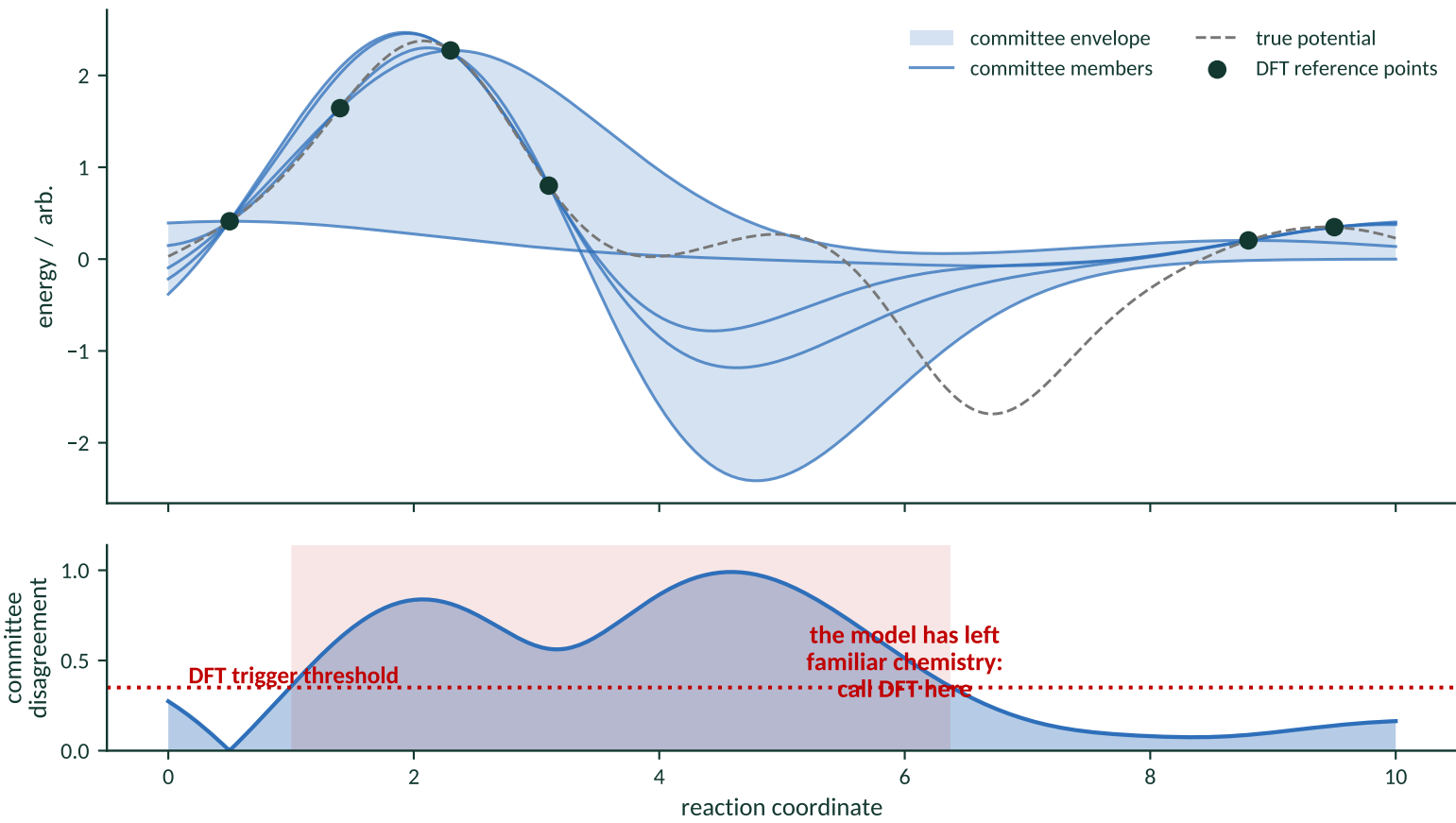
an ensemble of neural-network potentials, along one reaction coordinate
