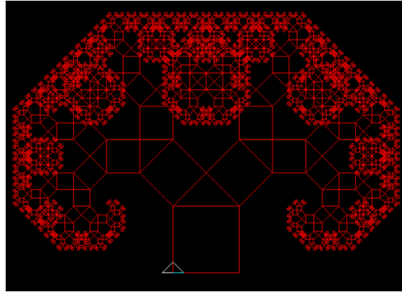
Pythagoras tree
