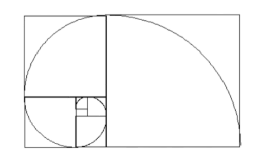
Golden ratio
