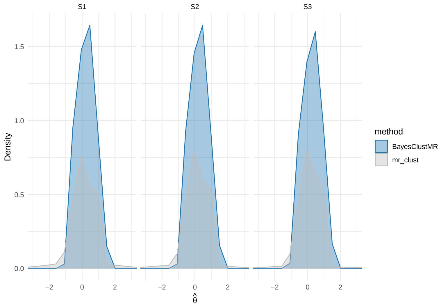
Density of \hat{\theta} by method
