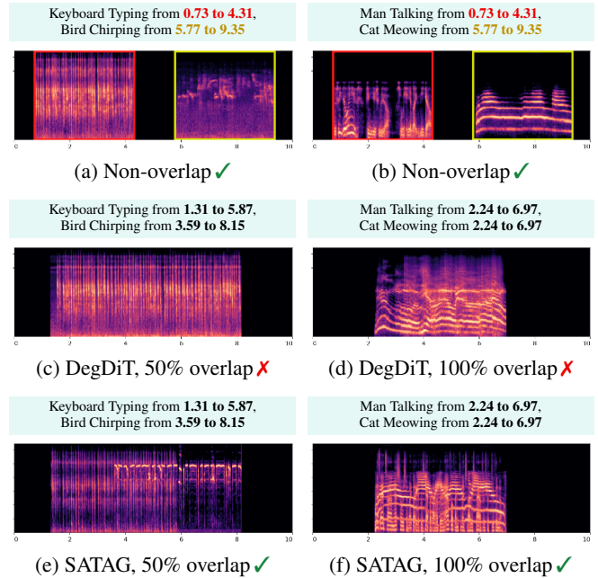
Fig. 1. Mel spectrograms of DegDiT (a–d) and SATAG (e–f).
