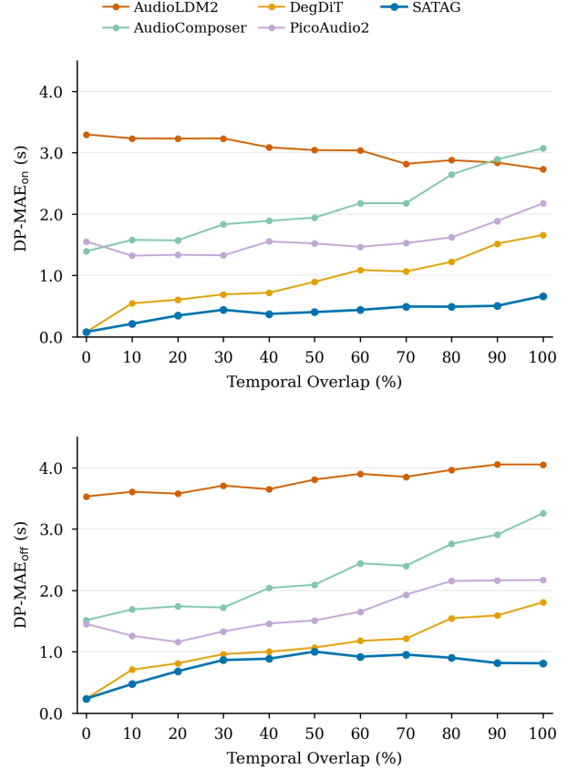
Fig. 3. Onset DP-MAE (top) and offset DP-MAE (bottom) across temporal overlap ratios for 200 event pairs.
