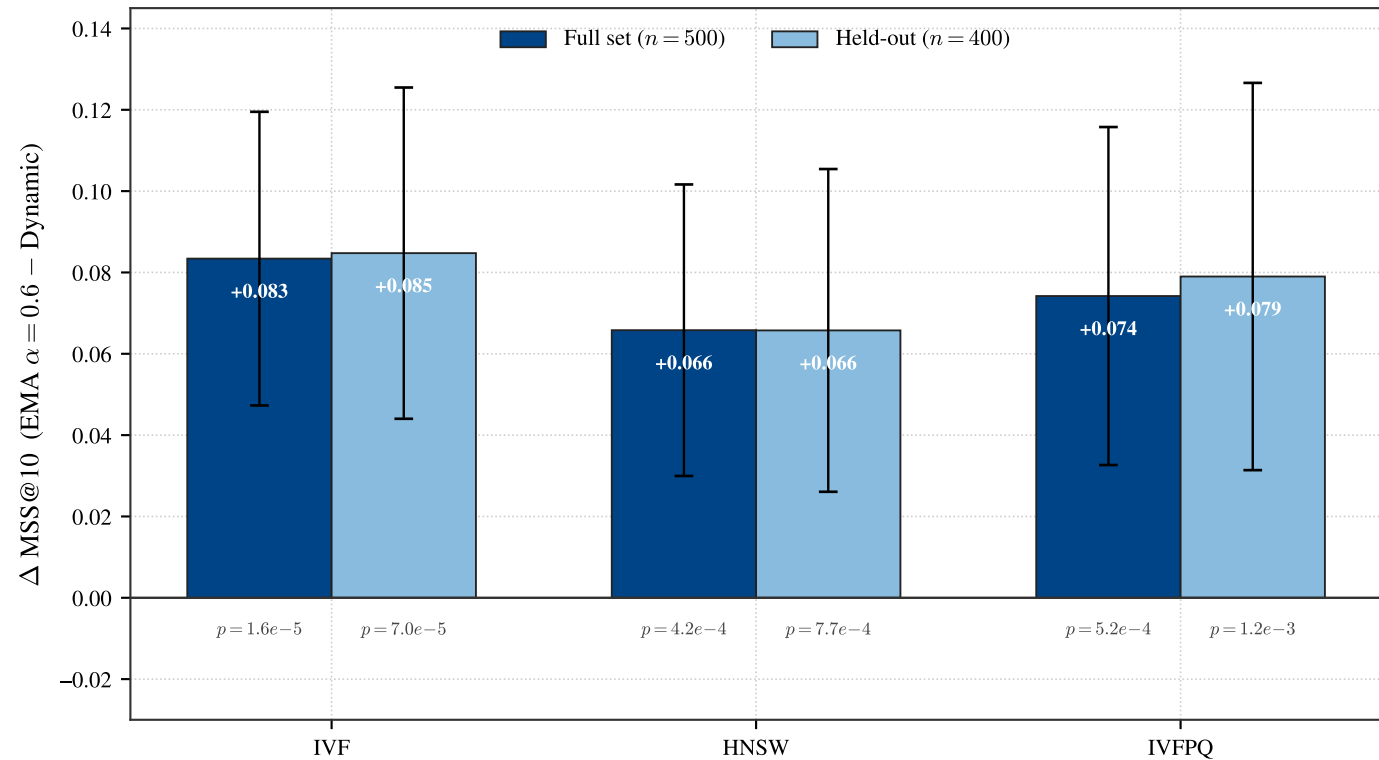
EMA improvement over Dynamic survives on held-out queries
