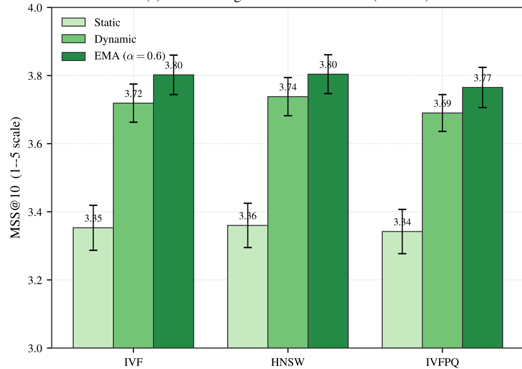
(a) Cross-dialogue filtered MSS@10 ( n = 500 )
