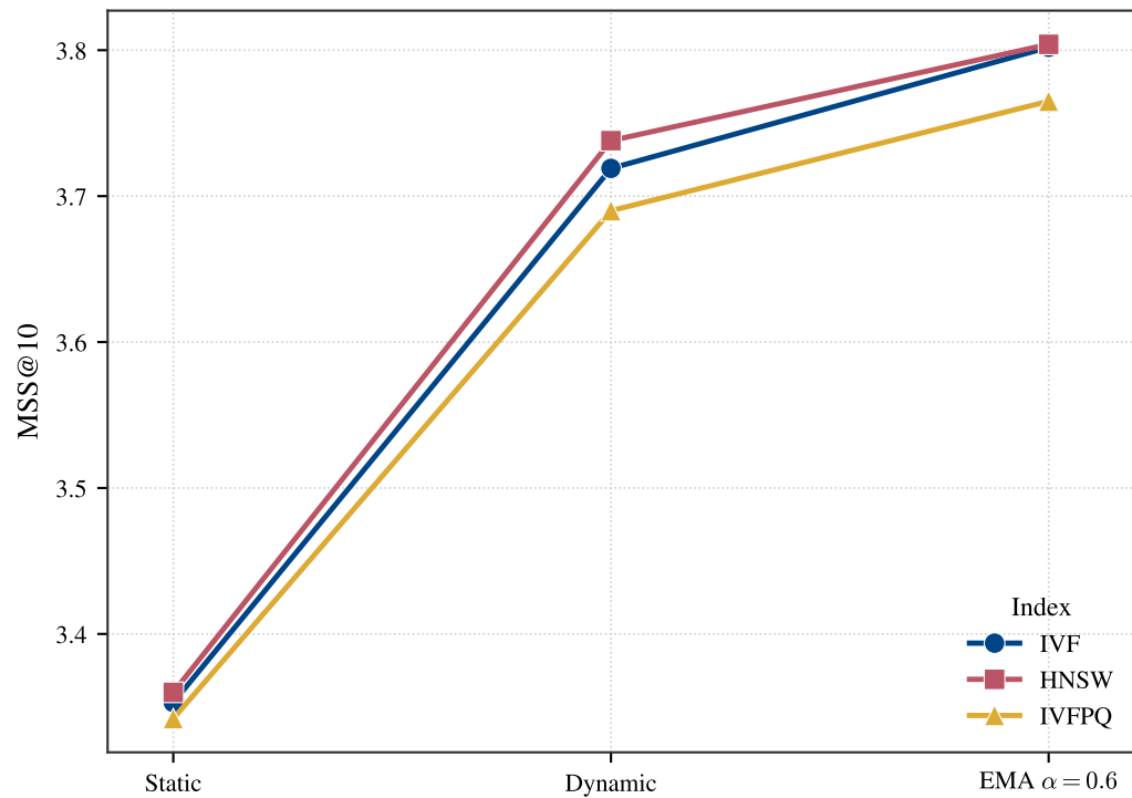
(b) Progression: static \rightarrow dynamic \rightarrow EMA
