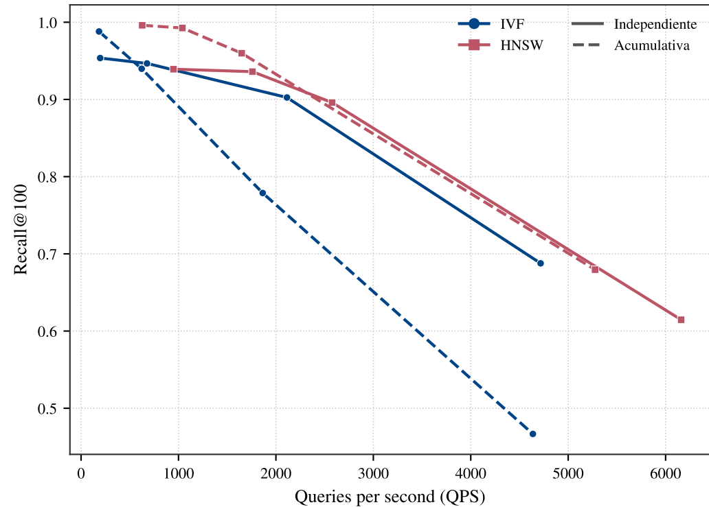
(a) Approximate retrieval over Dialog2Flow
