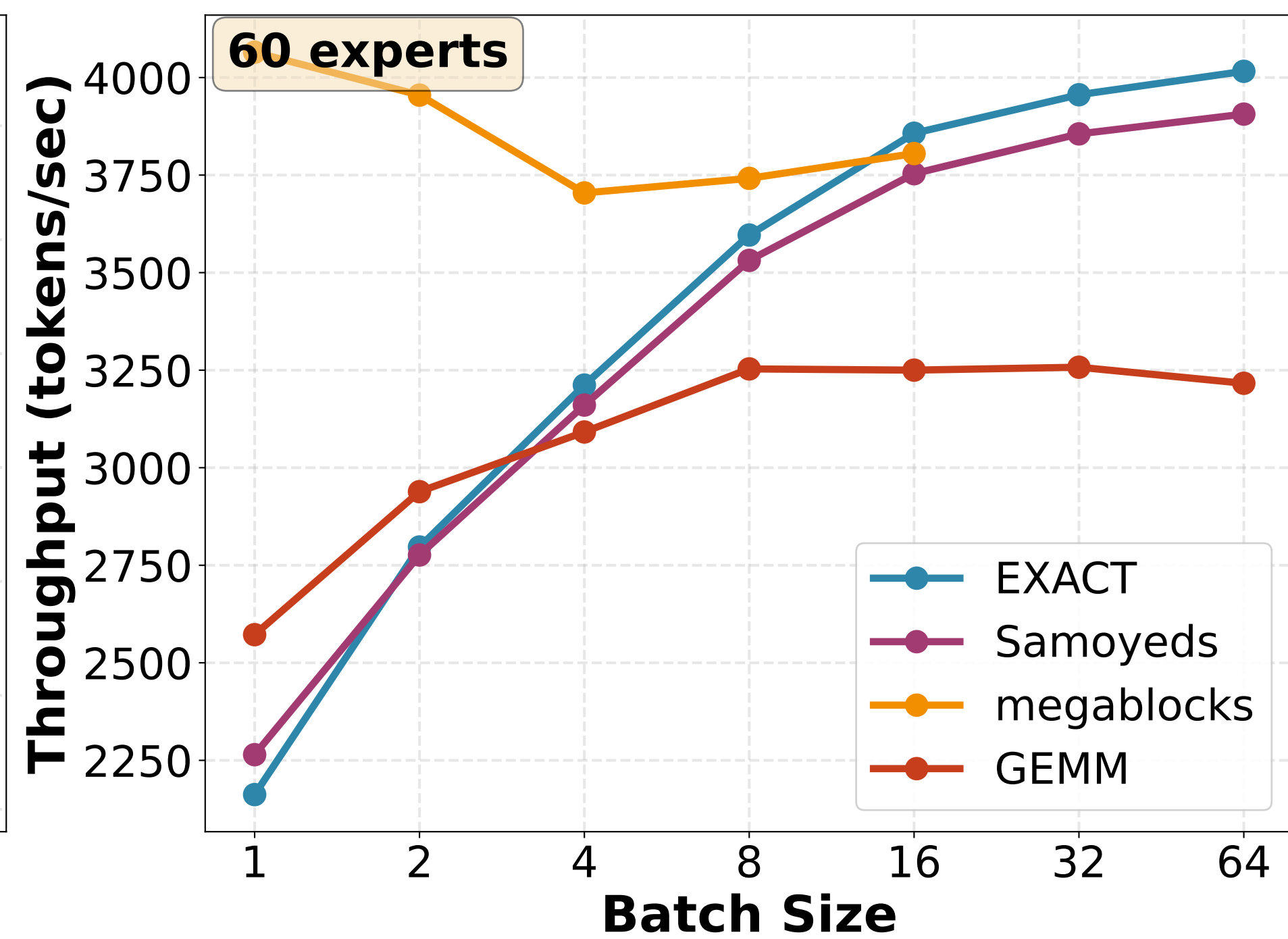
Qwen1.5-MoE-A2.7B
