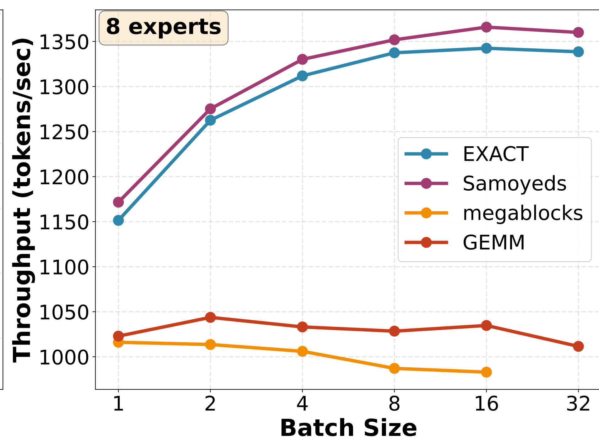
Qwen1.5-MoE-A2.7B
