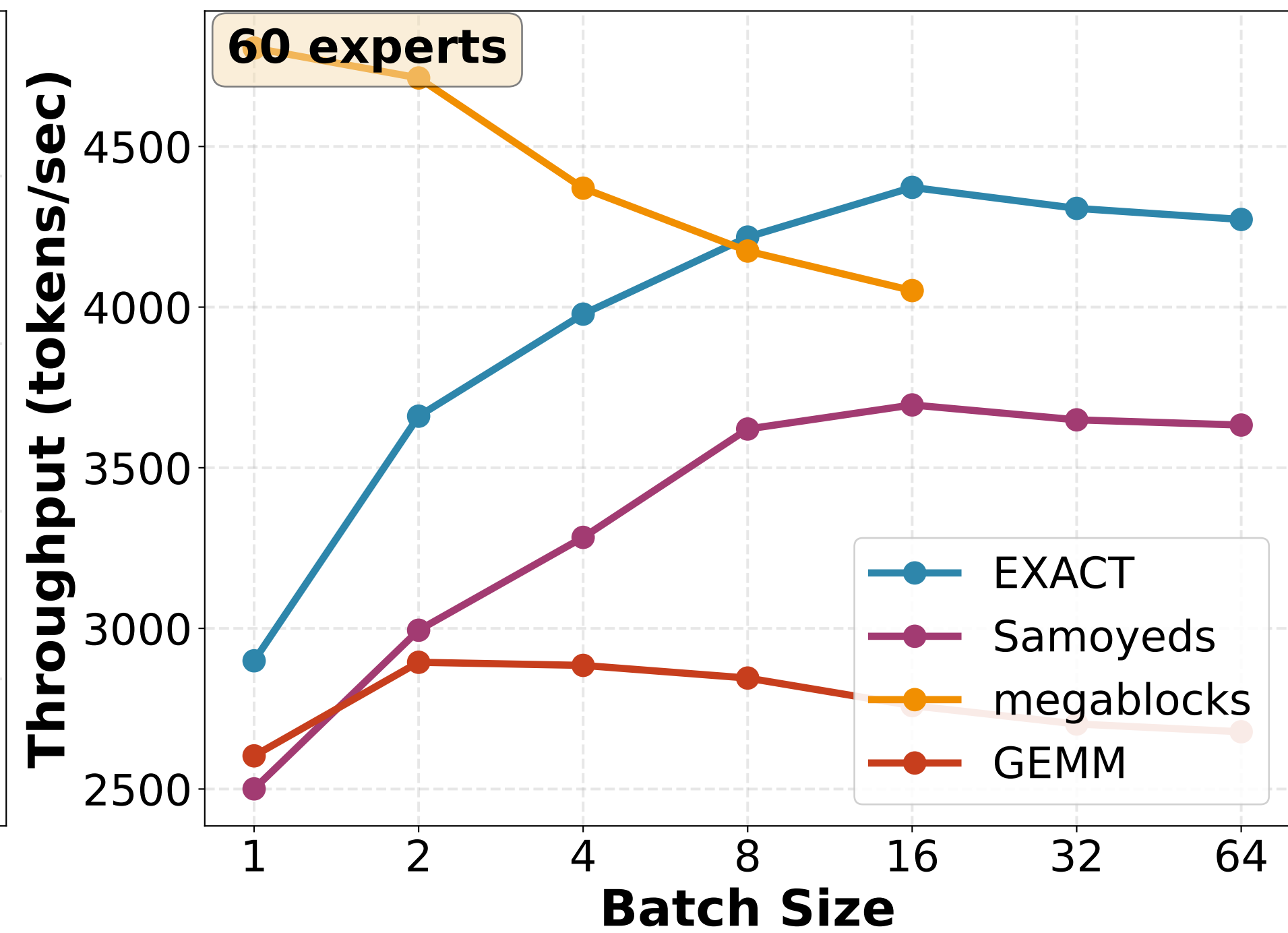
Qwen1.5-MoE-A2.7B
