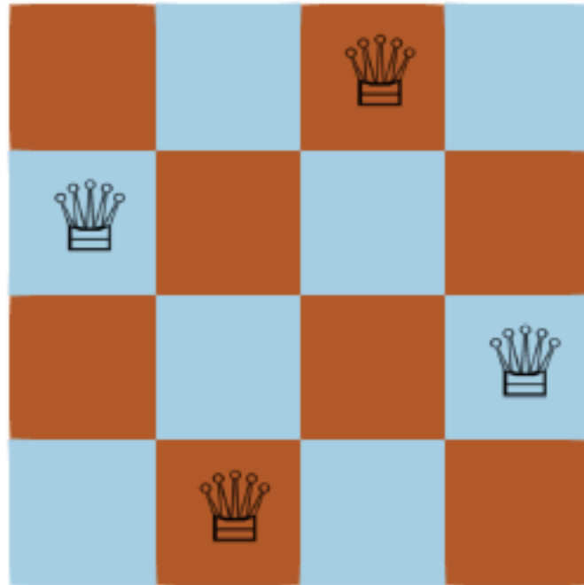
Figure 7.3: Four Queens
