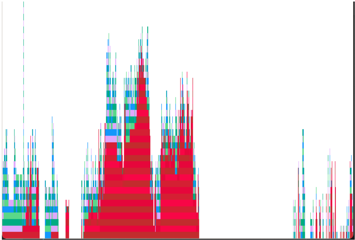
Figure 35.1: flamegraph
