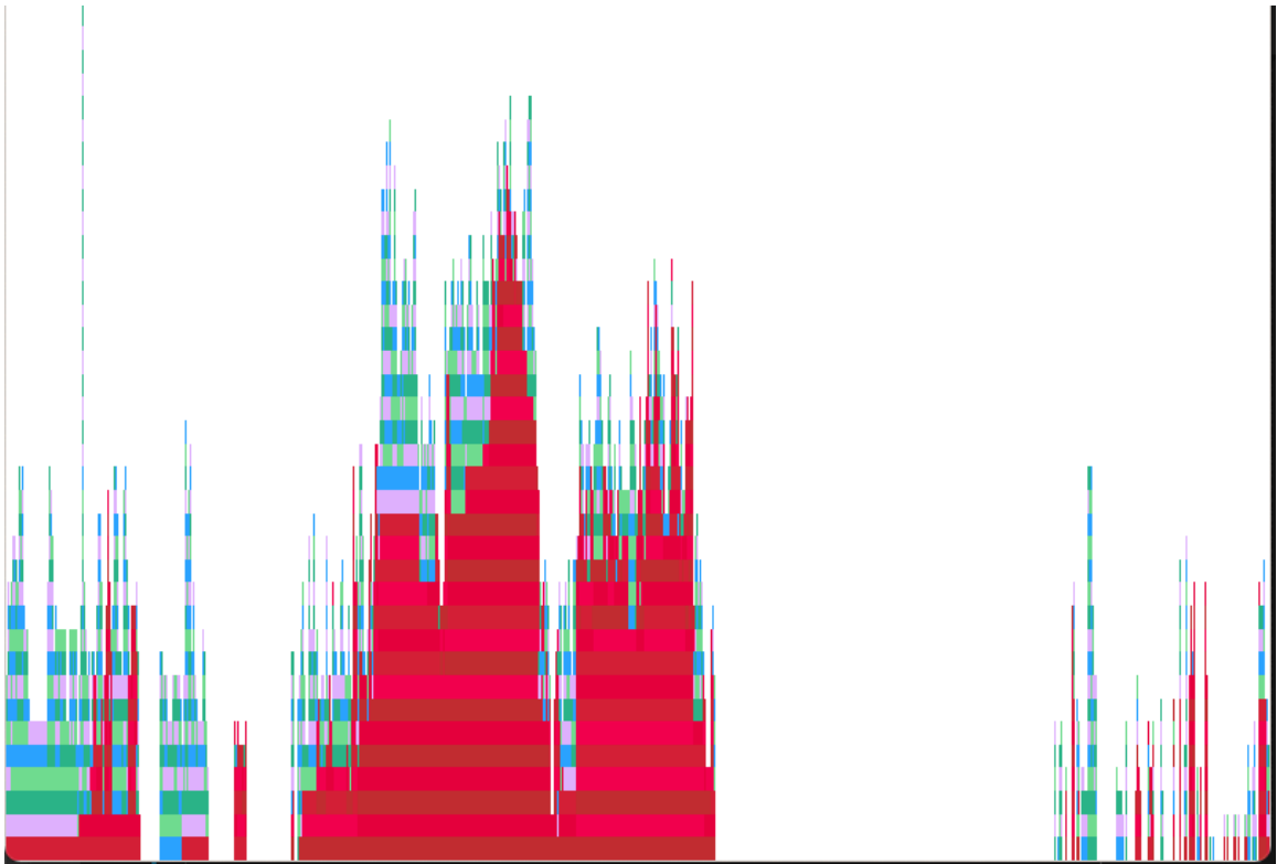
Figure 34.1: flamegraph
