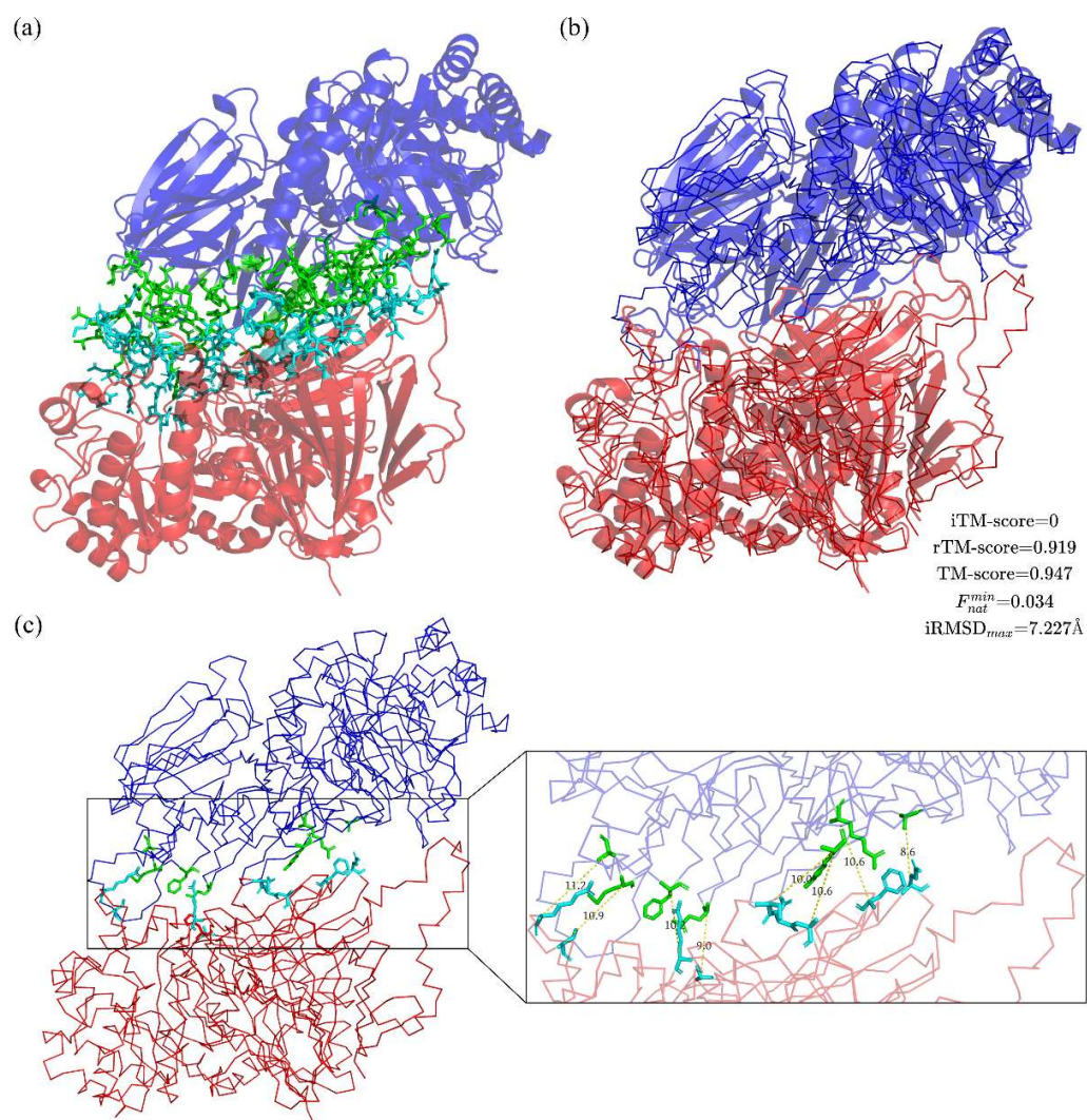
Fig. S2. Structure comparison between the predicted and native complex structures of PDB 2XN0. a. The native complex structure (cartoon) with interface residues (sticks). b. Superposition between the predicted (ribbon) and native (cartoon) complex structures. c. The predicted complex structure (ribbon) with the predicted interface, where the Ca distances of all predicted interface contacts are >8\text{\AA} . Each chain of the complex and the interface residues in different chains are shown in different color.
