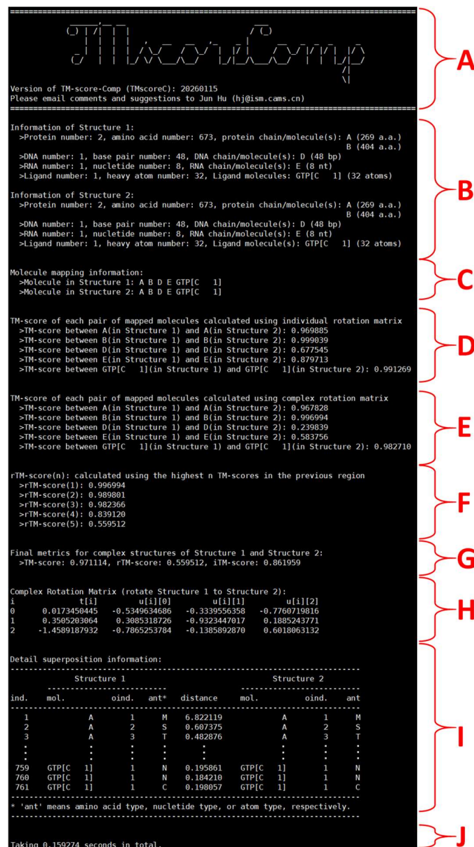
Fig. S6. Output example of the TM-score-Comp program. A. Program version and contact email. B. Inputted complex structure information. C. Molecule mapping result. D-E. single-molecule-level TM-scores calculated based on individual rotation matrix ( D ) and complex rotation matrix I . F. rTM-score( n ) calculated using the highest n TM-scores calculated based on complex rotation matrix. In order to evaluate the orientation quality of prediction model which missed one or more molecules, we have also demonstrated the rTM-score with different levels. The first level rTM-score, i.e., rTM-score(1), is calculated based on the highest single-molecule-level TM-score, the second level rTM-score, rTM-score(2), is calculated based on the highest 2 single-molecule-level TM-scores, and so on. G. TM-score, rTM-score and iTM-score for superposition between two inputted complex structure. H. Complex rotation matrix. I. Distances of superimposed residues/nucleotides/ligand atoms. 'ind.' Is line indexes, 'mol.' Is molecule information, 'oind.' Is original index in inputted PDB file, 'ant' is amino acid type, nucleotide type or atom type, 'distance' is the distance between two superposed residues/nucleotides/atoms In proteins/DNAs (RNAs)/ligands.
