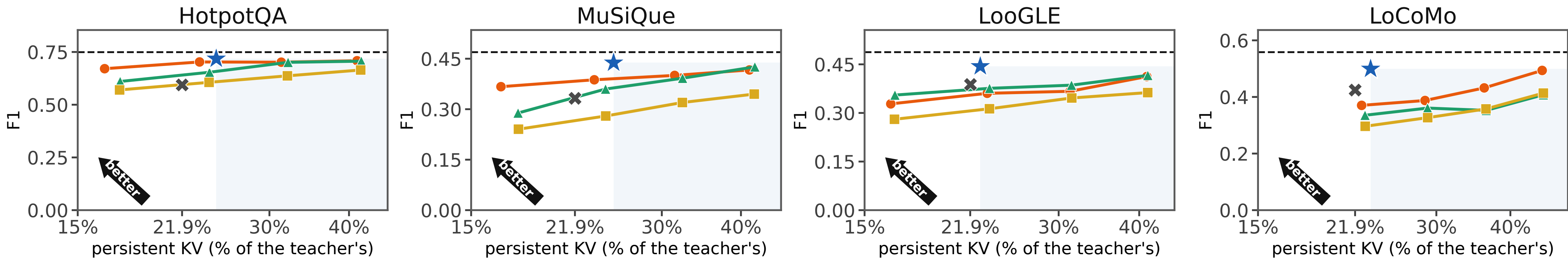
(a) accuracy against the persistent KV cache
