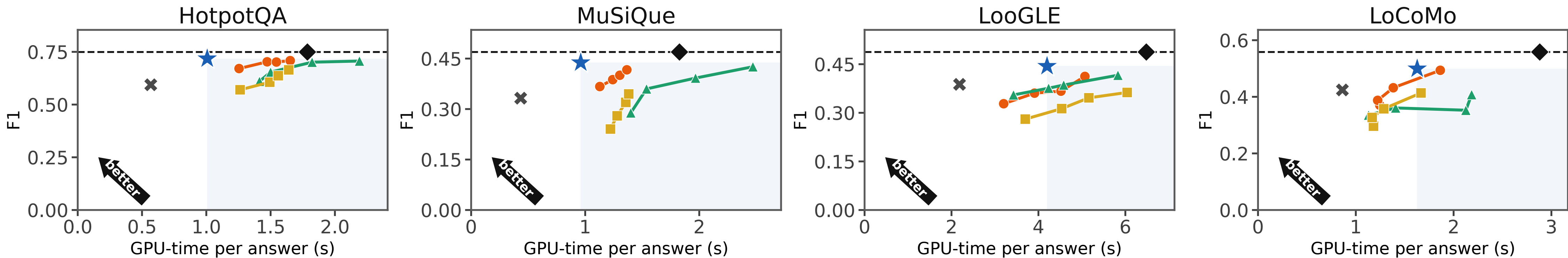
(b) accuracy against the GPU-time one answer costs
