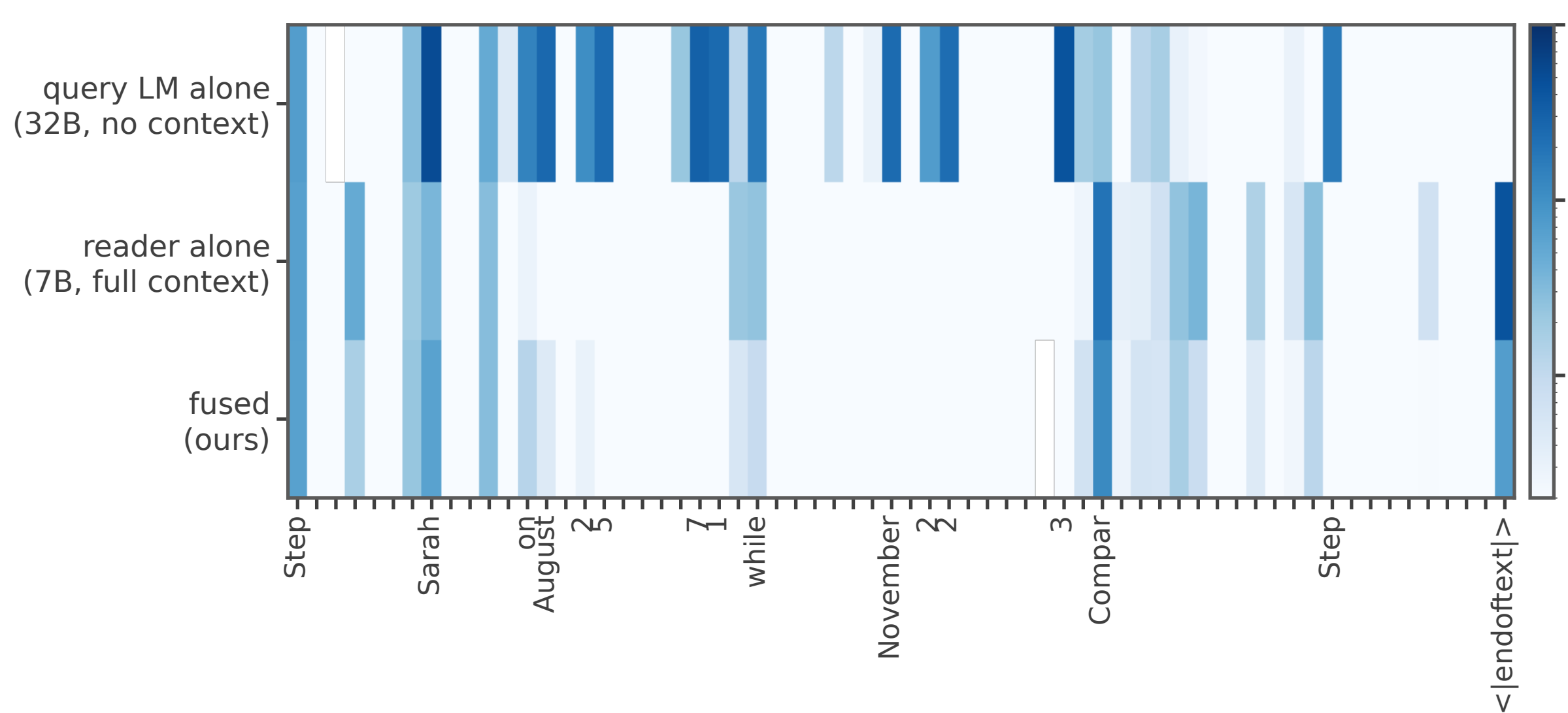
the teacher's answer, one token per column (a) one answer, token by token
