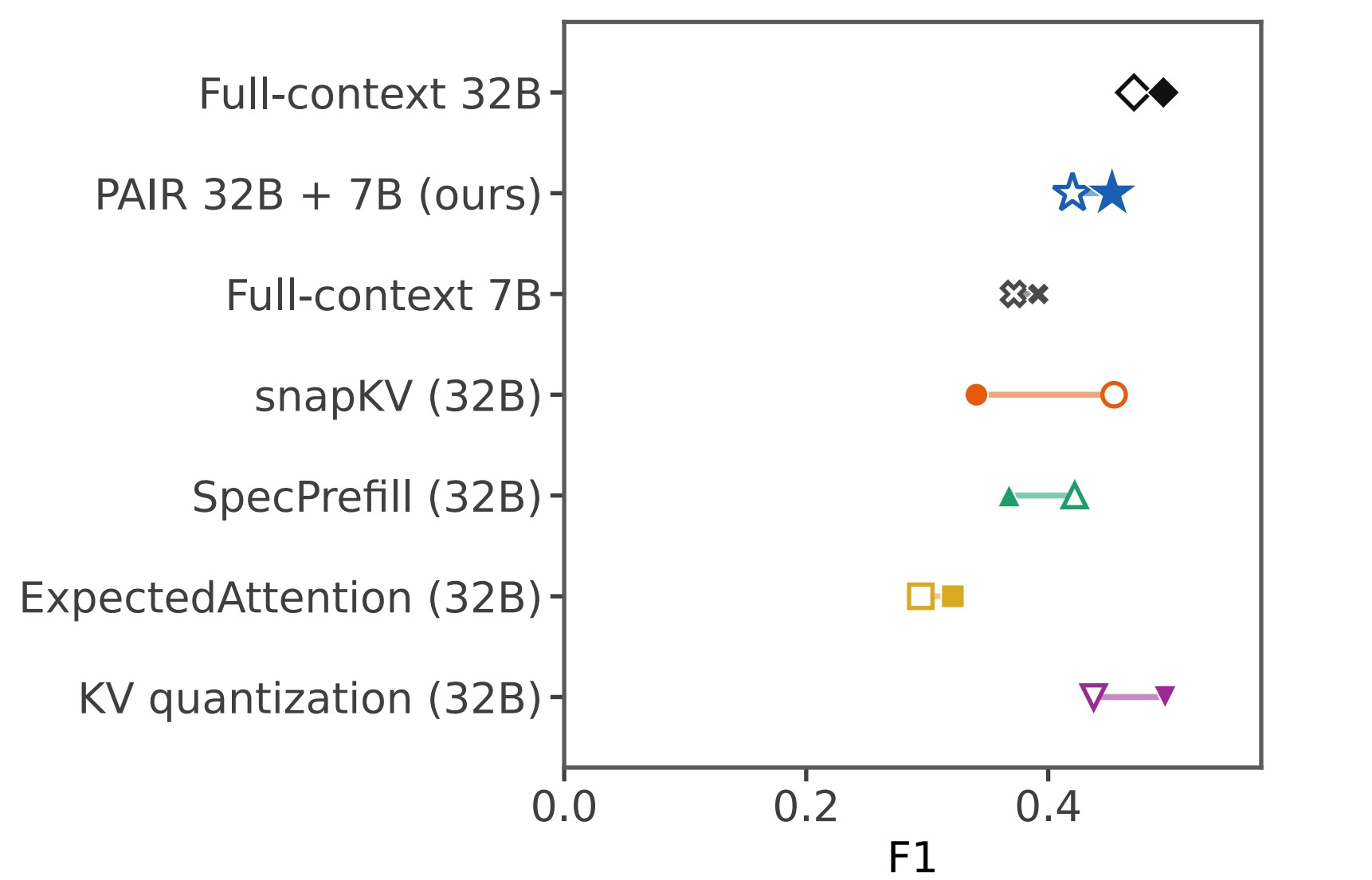
(c) LooGLE: first (hollow) vs later (filled)
