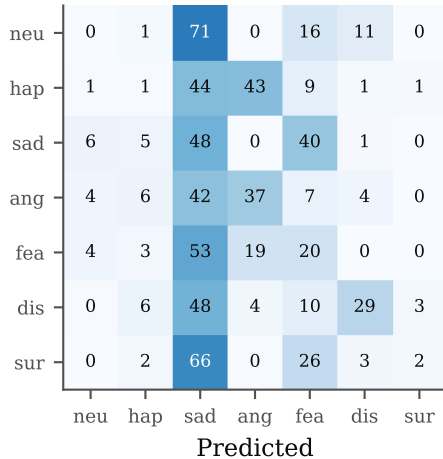
RAVDESS → TESS
