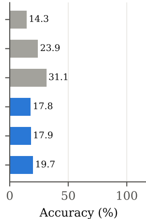
RAVDESS → TESS
