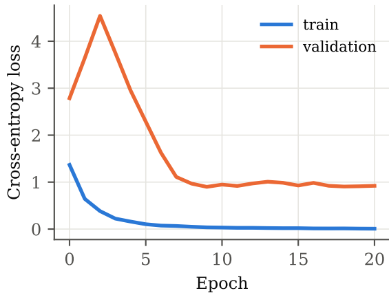
1D-CNN
