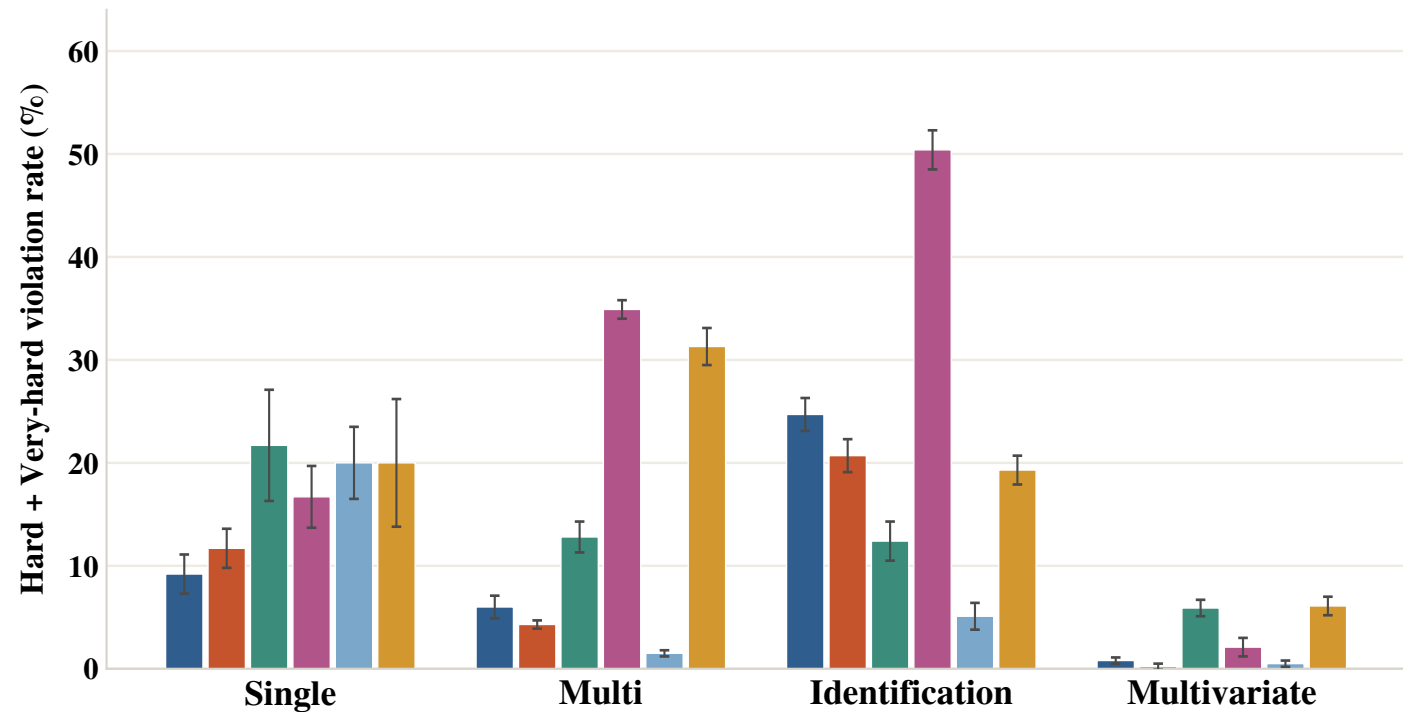
Violation rate by model and constraint type
