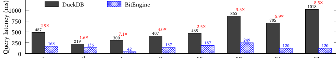
Figure 6: End-to-end latency on representative JOB queries. BITENGINE is faster on every query, by 1.6–8.5 \times (geomean 3.8 \times ), with the largest gains on the deep fact-fact join chains (26a, 31a). Rather than scanning the fact tables and building a large hash table per join as DuckDB does, BITENGINE evaluates each join as an FK-column predicate answered with bitmaps, then probes only the few surviving rows, orders of magnitude fewer than scanning/filtering the fact table (e.g., 33 of 36.2M in Q6c, Figure 7).
