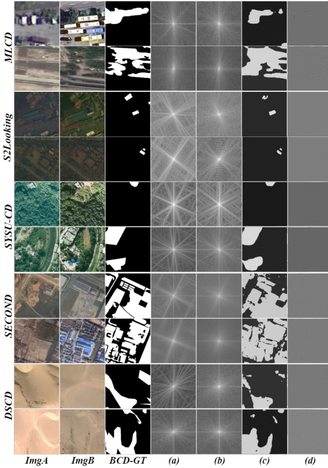
Fig. 11: Visualization of frequency-domain features and change information. (a) - (d) indicate FFT magnitudes of BCD-GT, FFT magnitudes of BCD-GT of prediction, low-frequency features of prediction, and high-frequency features of prediction, respectively.
