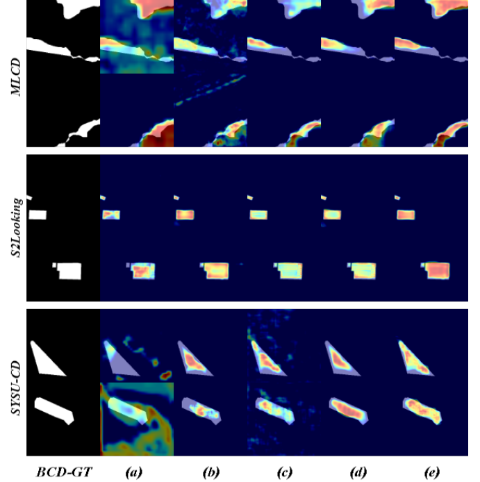
Fig. 7: The Grad-CAM visualization of BCD ablation studies. (a) - (e) indicate Baseline, +C&F, +LoRA, +BIFL, and FILFBCD, respectively.
