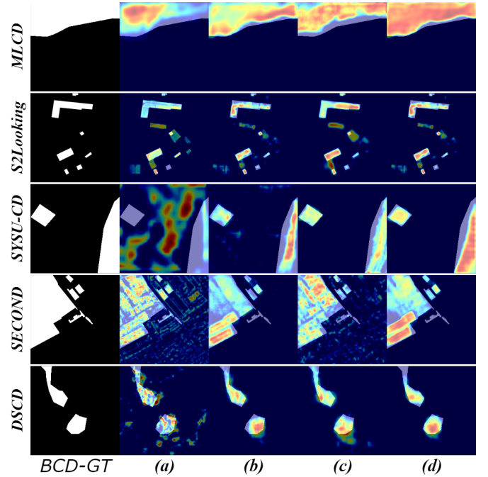
Fig. 10: Grad-CAM of difference feature domain comparison. (a) - (d) indicate ResBlock, Transformer, Mamba, and FFT(Ours), respectively.
