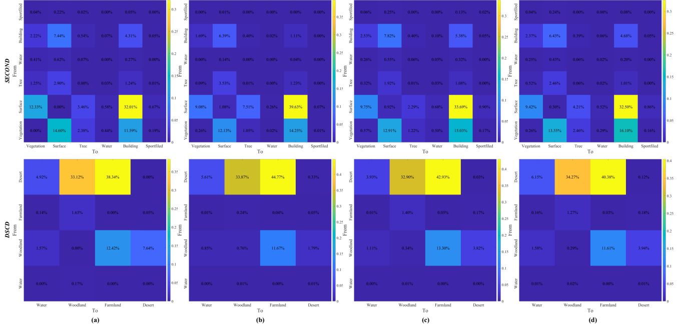
Fig. 9: Semantic change matrix providing “from-to” transition information derived from the ablation experiment results. (a) - (d) indicate reference, Baseline, +BIFL, and FILFSCD, respectively.
