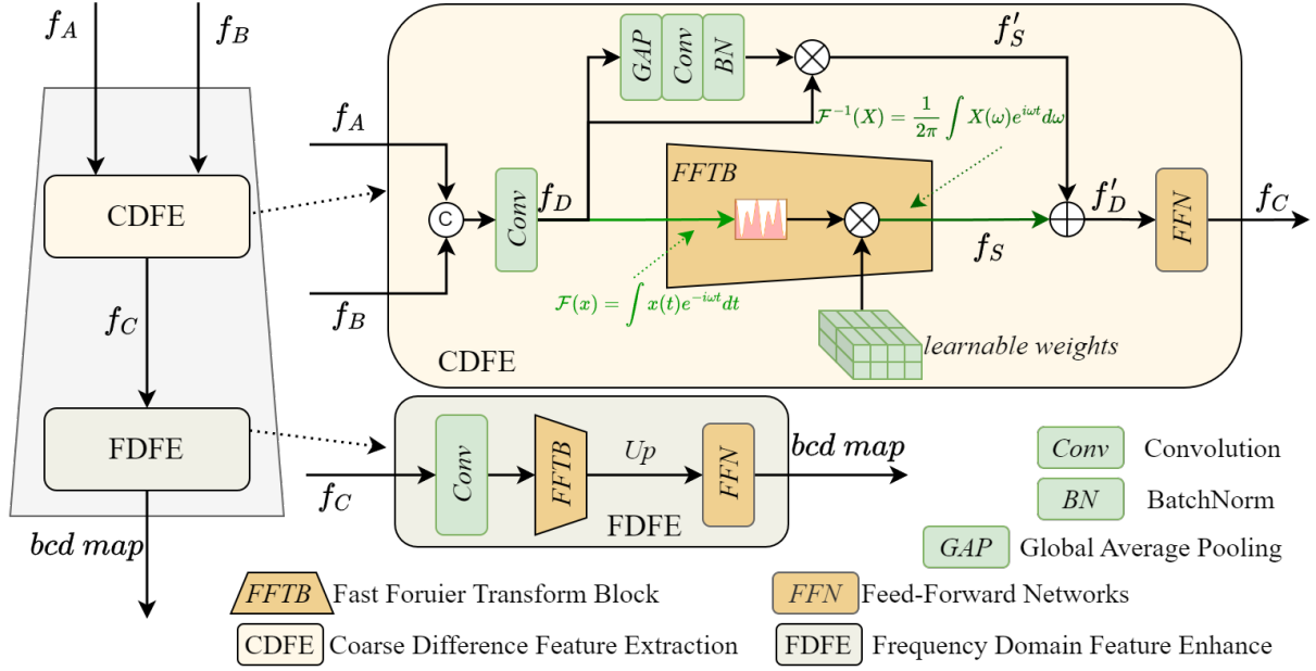
Fig. 3: Structure of the proposed BCD Decoder, which consists of the Coarse Difference Feature Extraction (CDFE) and the Frequency Domain Feature Enhance (FDFE). The CDFE compares bi-temporal features by first mapping them into the frequency-domain via the FFT. It analyzes multi-scale feature differences in frequency-domain to generate coarse-grained change features. The FDFE utilizes the FFTB to convert low-resolution change features from spatial to frequency-domain. By capturing multi-scale and long-range contextual information, it enables more accurate feature recovery through global dependency modeling.
