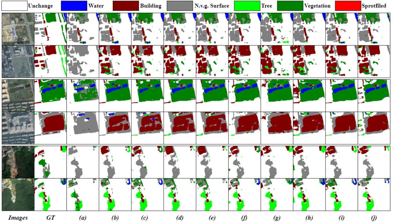
Fig. 5: Visualization of SECOND. (a) - (g) indicate SSCDI [39], BiSRNet [39], SSESN [84], CdSC [40], MambaSCD [55], SCD-SAM [66], and SAM-FE [85], respectively. (h) - (j) indicate our proposed FILFSCD (ViT-H), FILFSCD (Tiny-ViT), and FILFSCD (Hiera-Large), respectively.
