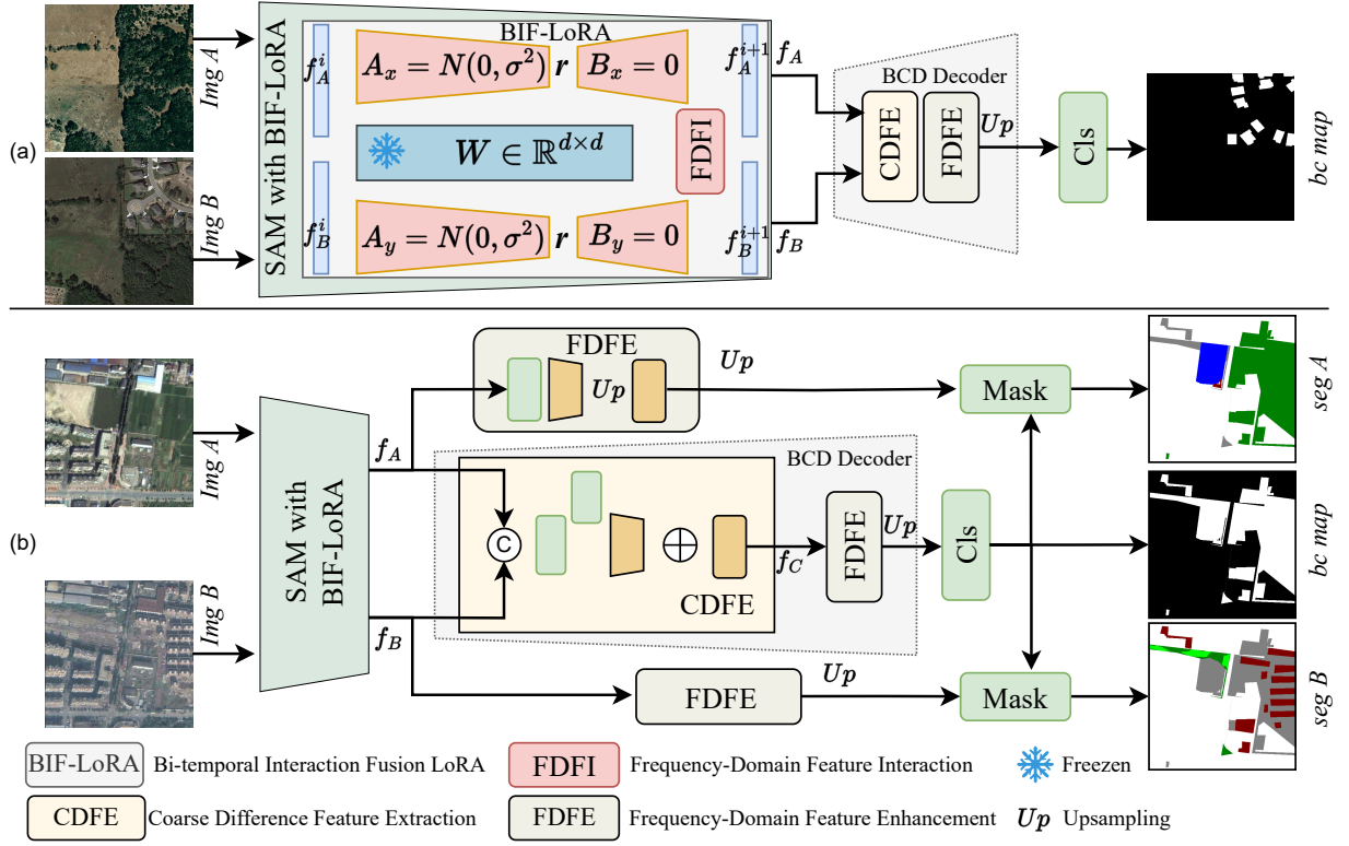
Fig. 1: Structure of the proposed FILFArch, where (a) shows the FILBCD for BCD and (b) shows the FILFSCD for SCD. In FILFArch, to enhance the capability of SAM in extracting cross-temporal remote sensing features while reducing training weights, BIF-LoRA is designed to extend LoRA to bi-temporal feature processing. BIF-LoRA employs frequency-domain guidance to fuse cross-temporal correlated features, thereby strengthening the extraction of change-related features. The BCD Decoder consists of the CDFE and FDFE. The CDFE performs an initial fusion of bi-temporal feature differences to generate coarse-grained change features. The FDFE leverages frequency-domain guidance to restore refined feature representations. Meanwhile, the FDFE is also utilized to semantic features recovery in FILFSCD.
