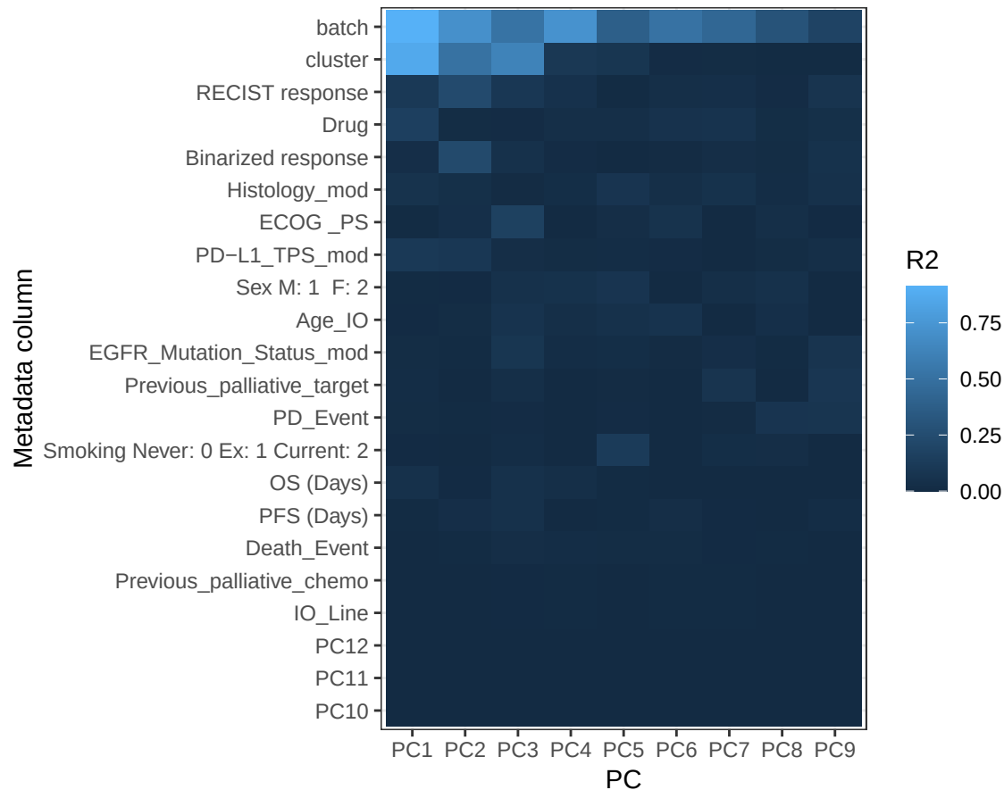
How strongly each PC is associated with each r
