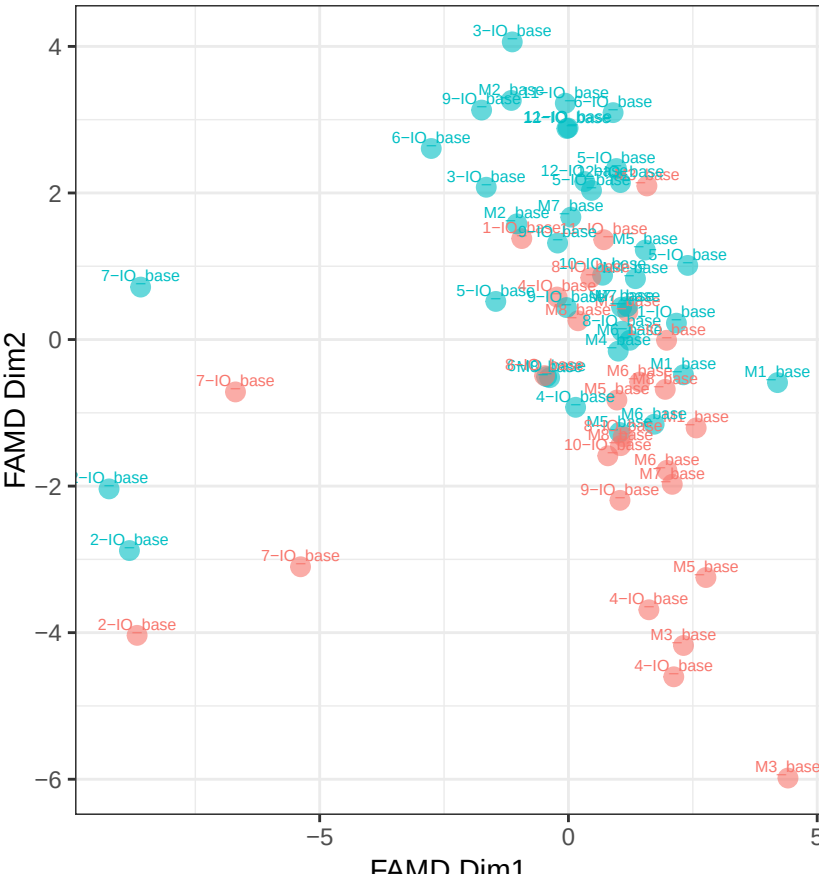
FAMD plot
