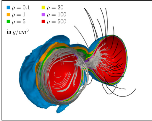
Figure 1. The figure shows an exploded view of the internal structure of a double white dwarf binary star system during the mass transfer phase that precedes the eventual merger of the two stars into a single object. Color is used to indicate density layers ( 0.1 to 500 \text{ g/cm}^3 ). The star to the right of the image (the donor) is transferring mass through a stream striking the upper layers of the more massive white dwarf to the left (the accretor). Several pathlines (gray) show how the stream impacts the accretor, with most of the mass flowing around the accretor while some fraction of the stream spreads in all directions around the point of impact.
