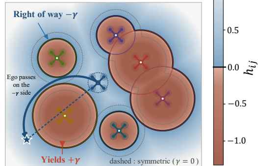
(c) Precedence-encoded CBF
