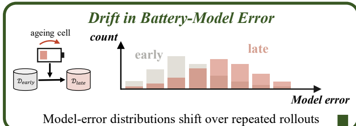
(a) Adaptive calibration under battery model-error drift
