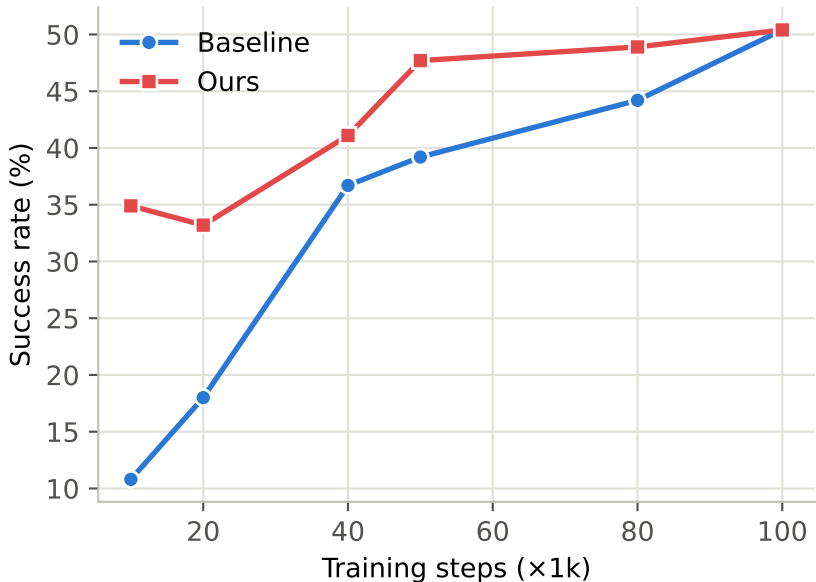
Dit4Dit Video-frozen From-Scratch GR-1 Tabletop 1000 demos
