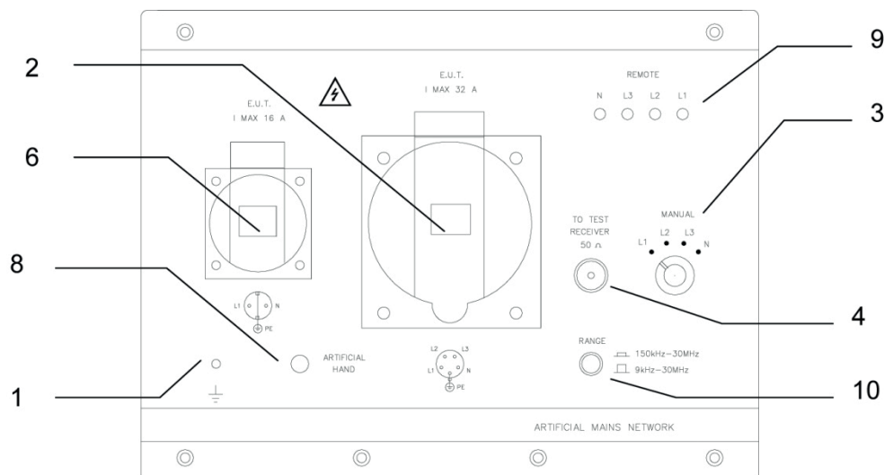
Fig. 2-1 Front Panel
