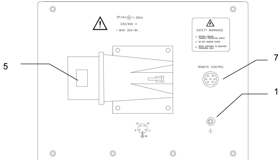
Fig. 2-2 Rear Panel
