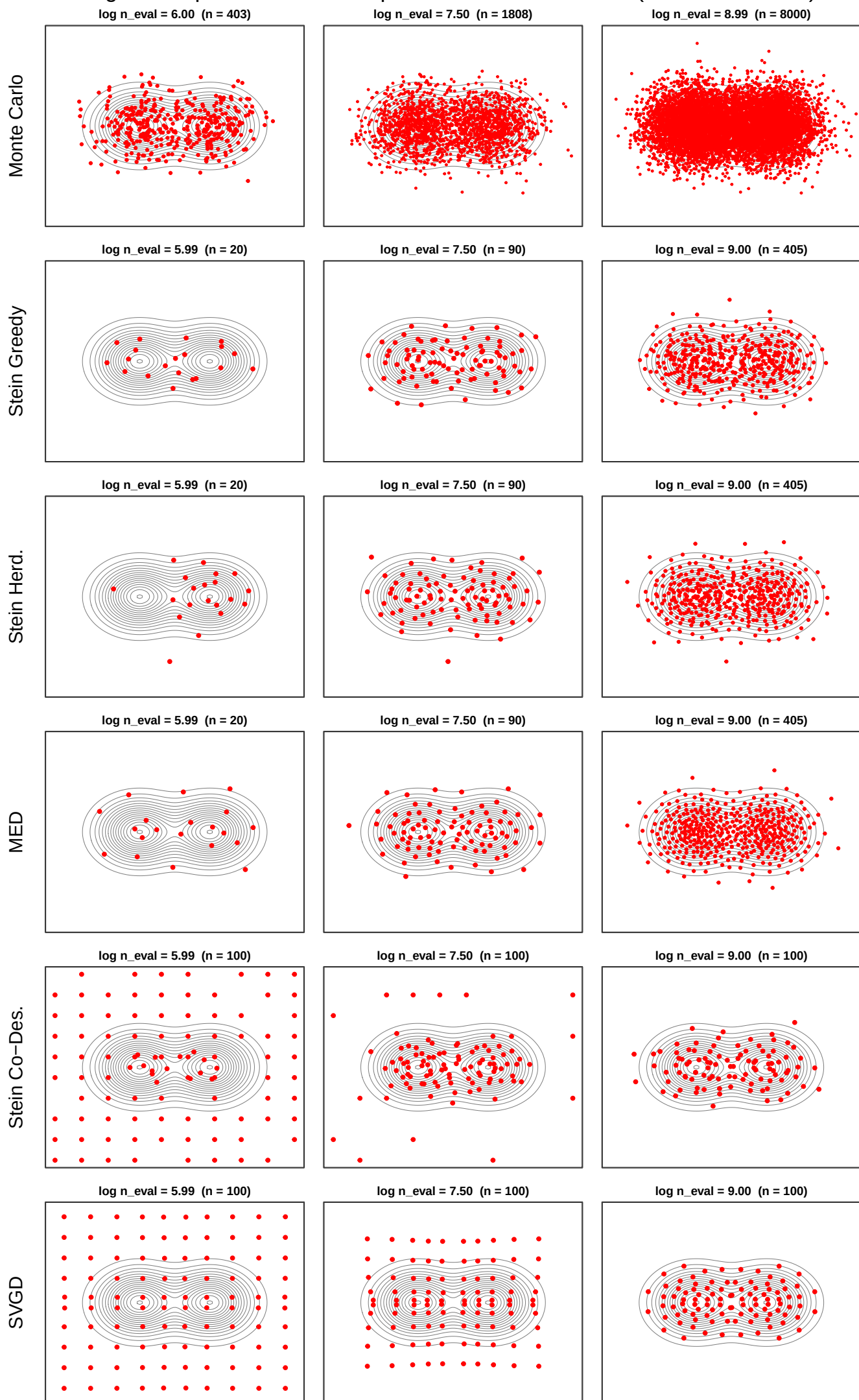
Figure 1 reproduction: 2-component Gaussian mixture (Chen et al. 2018)
