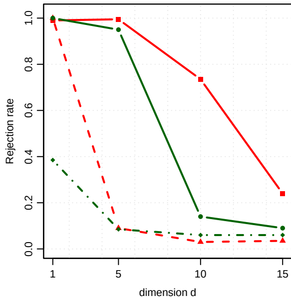
(a) Gaussian vs. Laplace
