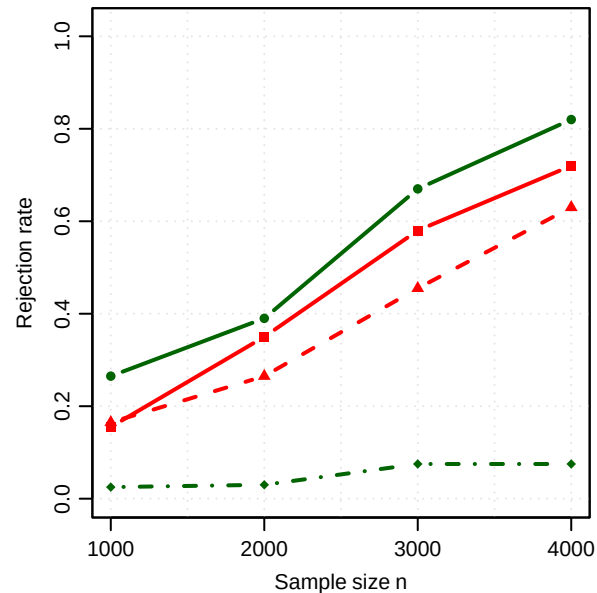
(c) RBM, perturb B[1,1]
