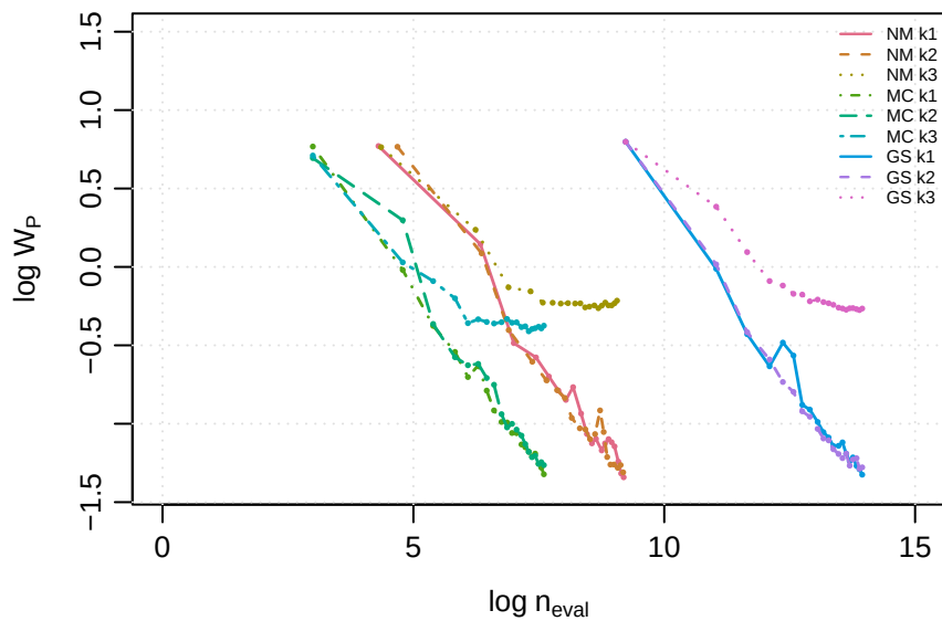
(a) Stein Points (Greedy)
