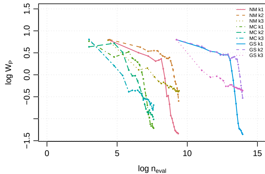
(b) Stein Points (Herding)
