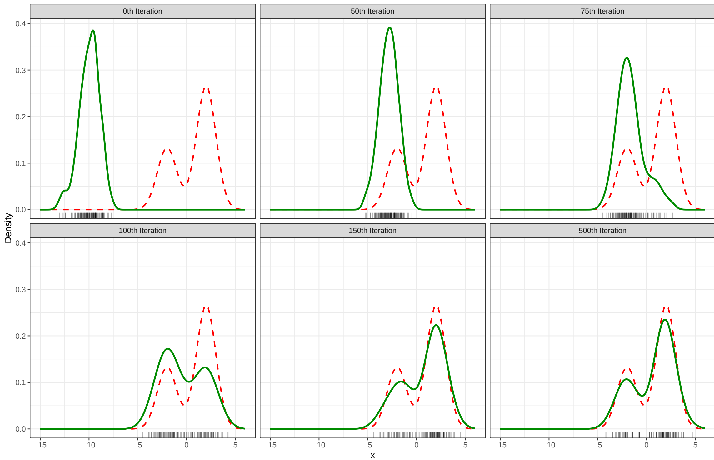
Figure 1: Toy example with 1D Gaussian mixture
