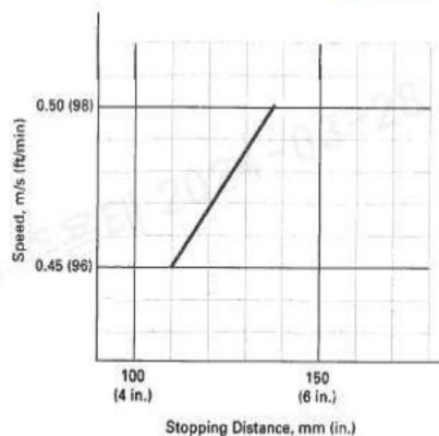
Figure I-11 Stopping Distances Corresponding to a Deceleration Rate of 0.91 \text{ m/s}^2 [6.1.5.3.1(c)]
