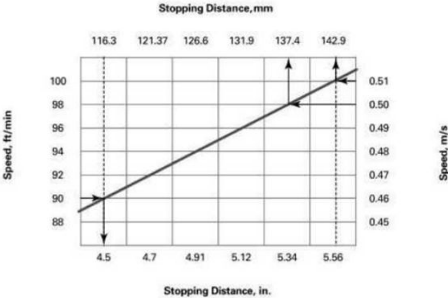
Diagram 6.1.5.3.1(c) Escalator and Moving Walk Stopping Distances
