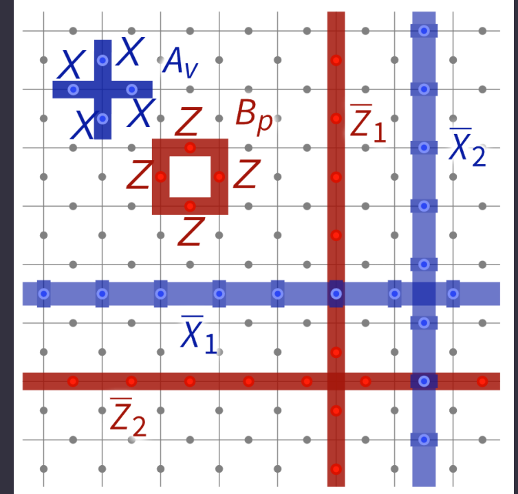
Fig. Toric code [Kitaev, 1997] (from EC Zoo)
