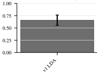
All-trial accuracy
