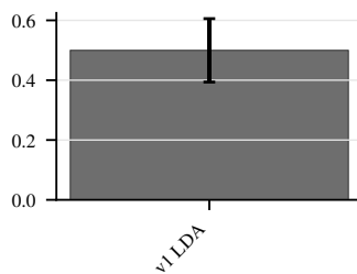
Brier score
