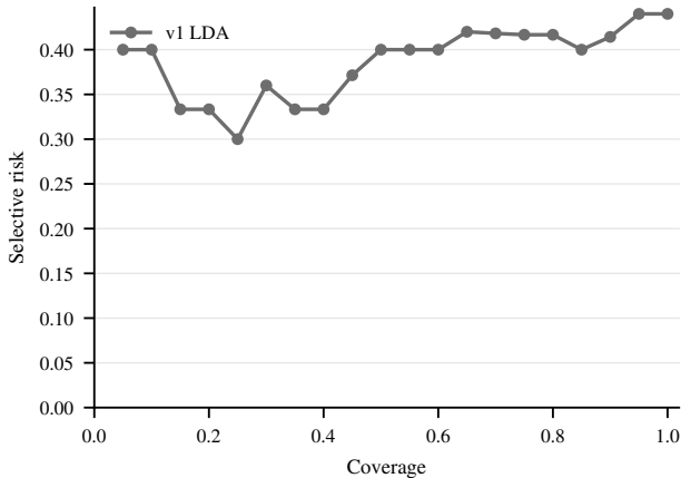
PhysioNet MI: risk-coverage
