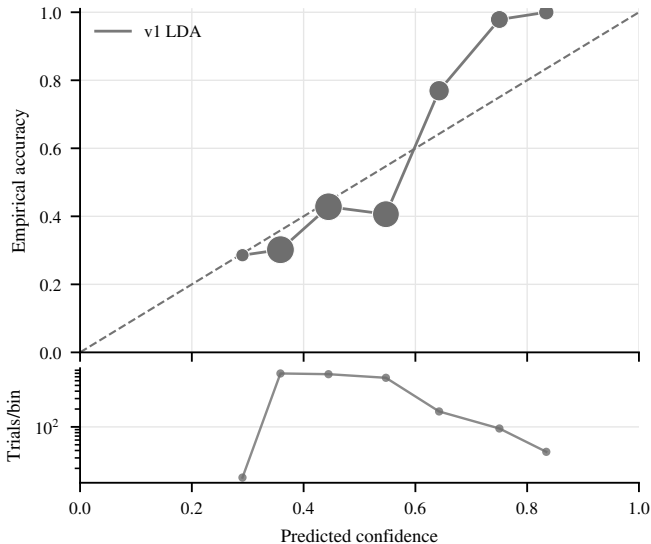
BCI Competition IV 2a: trial-weighted reliability
