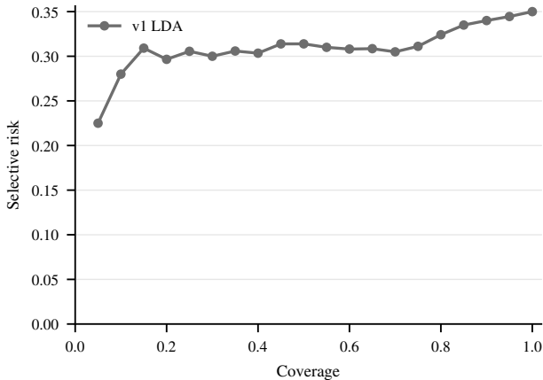
BNCI 2014-001: risk-coverage
