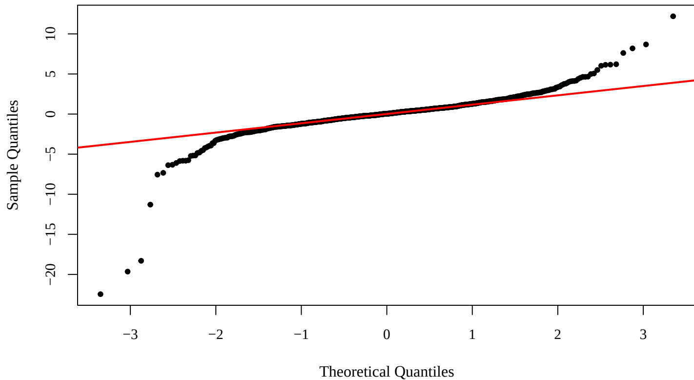
Q-Q Plot of FF5 Residuals
