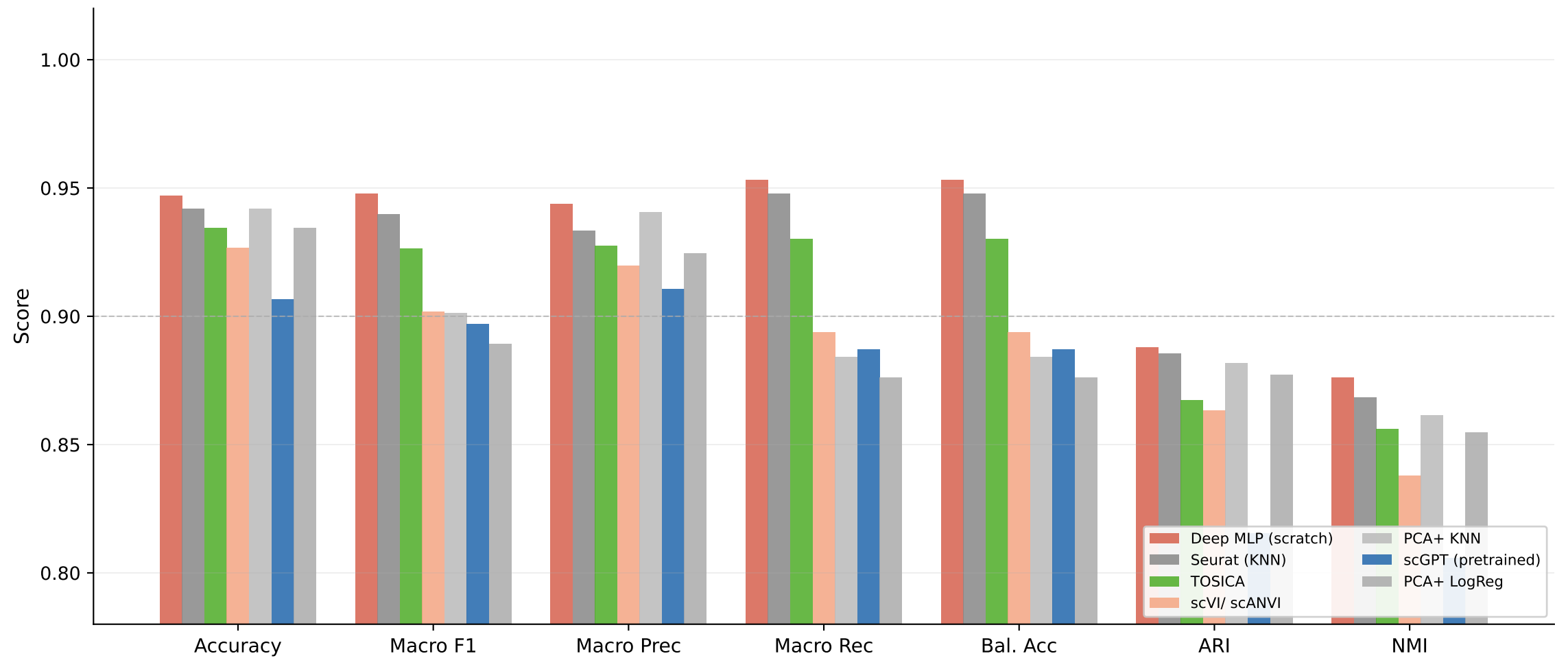
All Metrics Across All Methods — PBMC3k Benchmark
