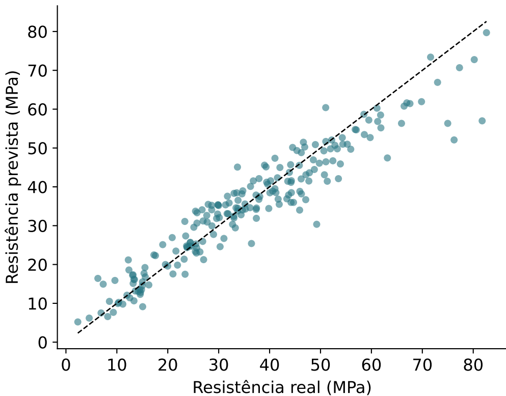
Baseline — holdout
