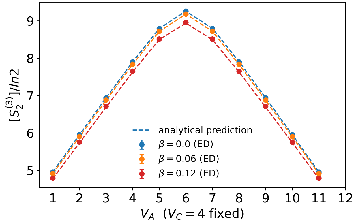
(a). maximally chaotic ( g = 1.1, h = 0.35 ), V = 16
